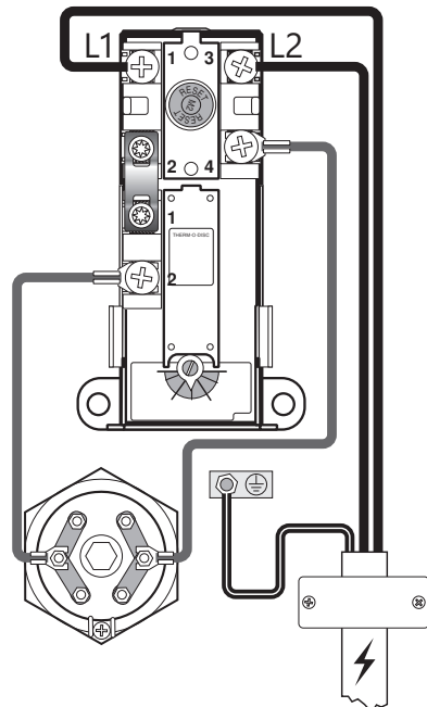
Electrical connection 4,8 kW
