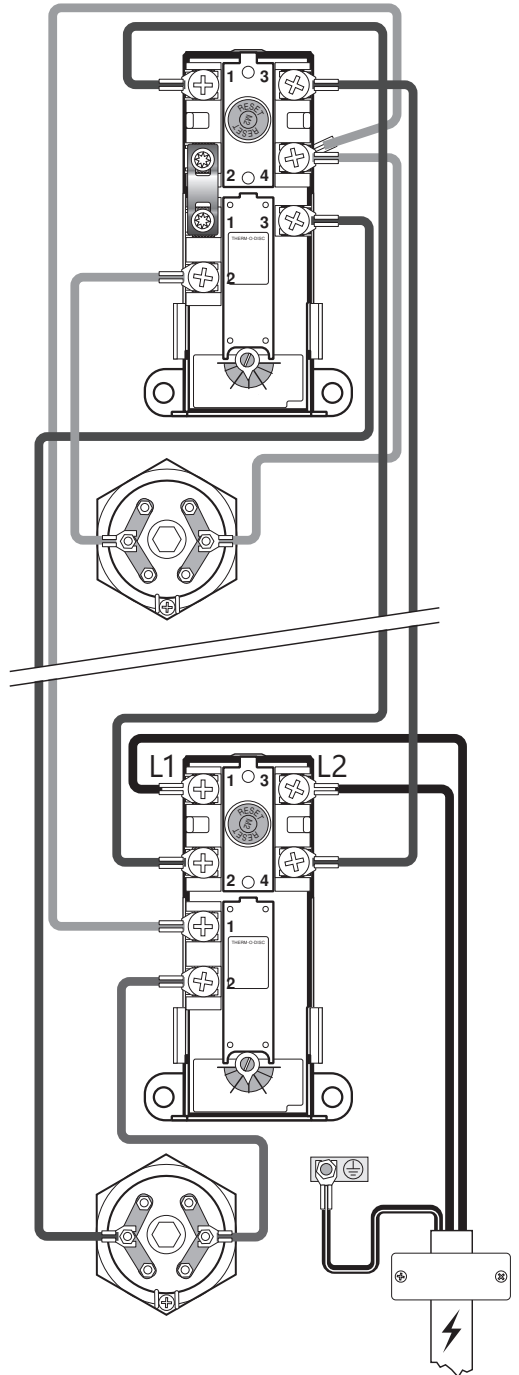
Electrical connection, diagram 4,8+4,8 kW
